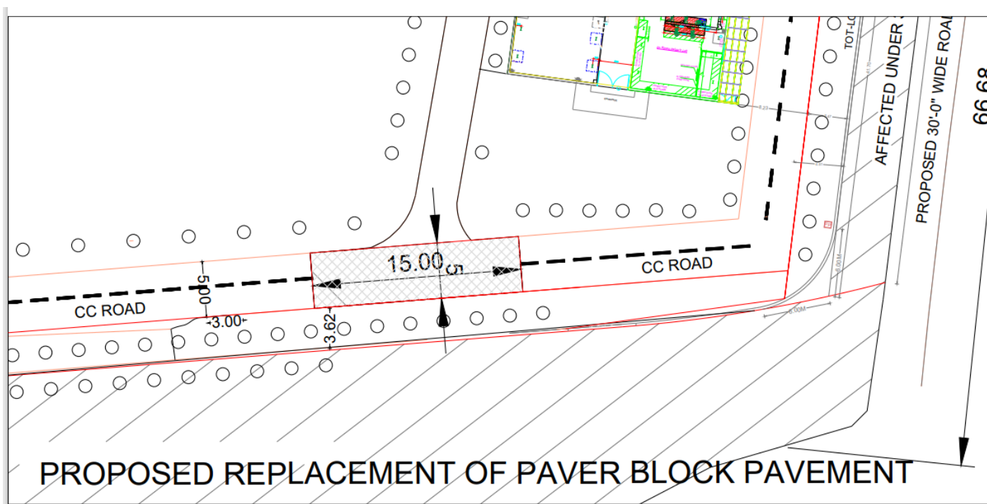
Proposed paver block pavement replacement plan
